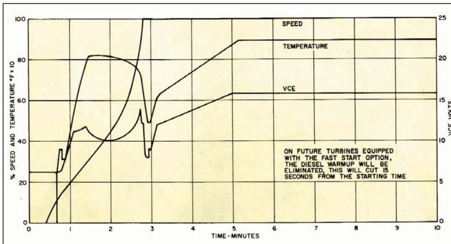
Figure 1: Above are starting and loading graphs derived from data recorded on frame 7. Maximum exhaust temperature during startup was 810°F
